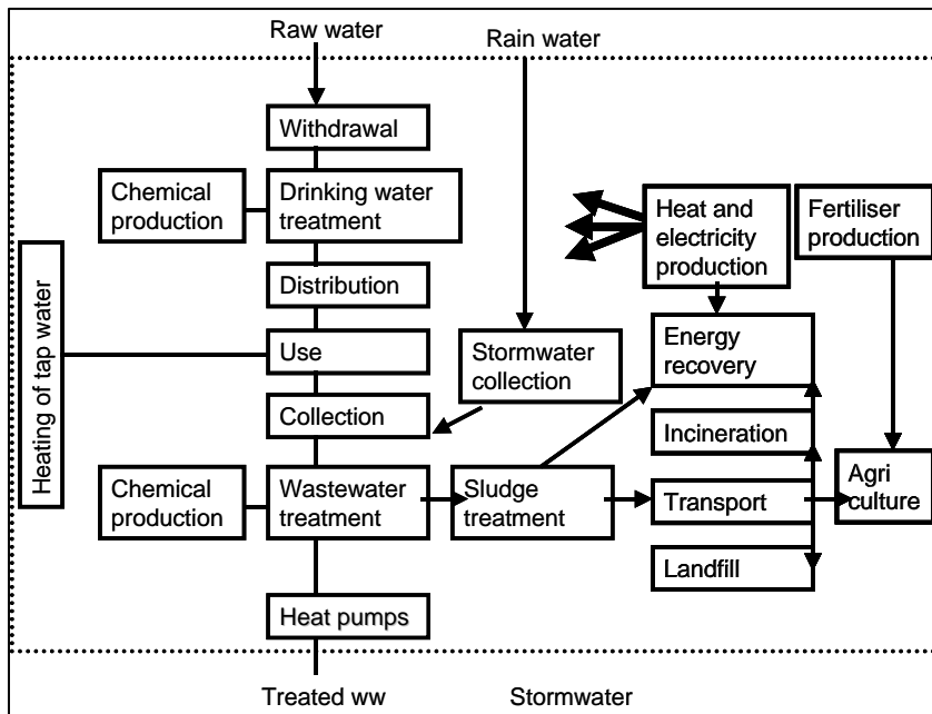
Figure 7.5: Urban Water System From Lundin and Morrison (2002) (Source: Peter van der Steen, 2006)
